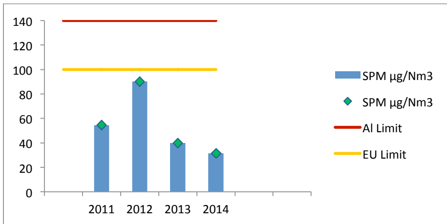
Graph No. 4: SPM emissions
