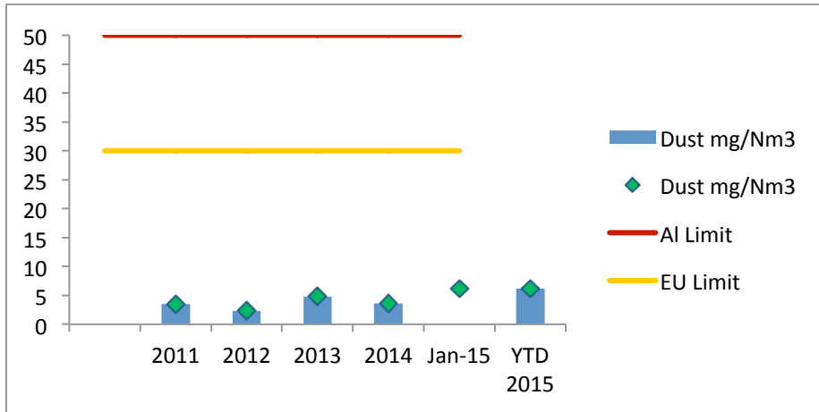
Graph No. 3: Dust emissions from kiln
